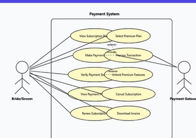
Payment & Subscription System
